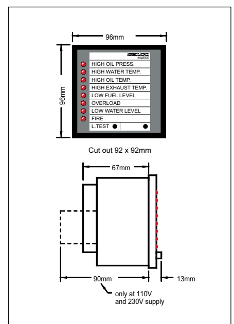
M4600 dimensions.
