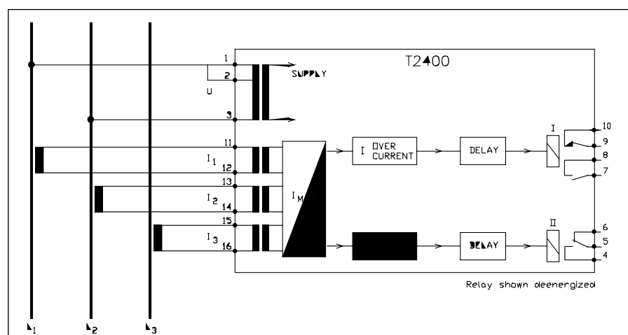
Connection diagram.
